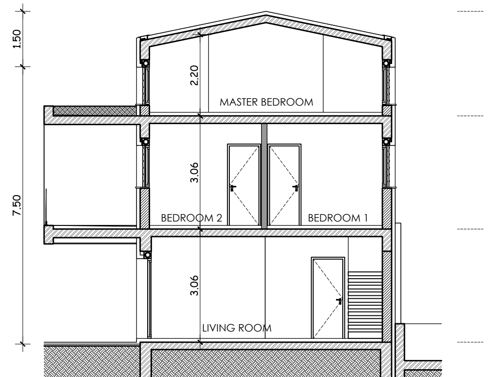
SECTION T2
