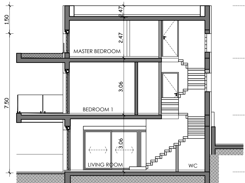
SECTION T1
